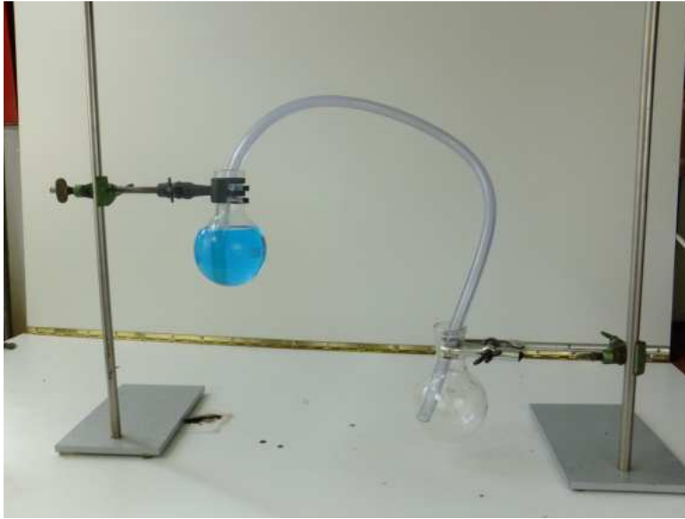
Abb. 6: Das Saugheber-Modell
